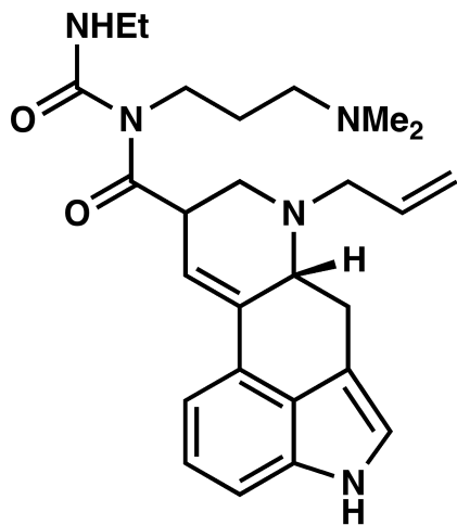
cabergoline
