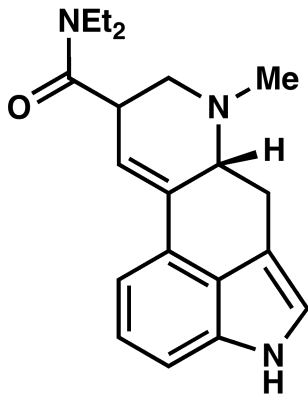
LSD
