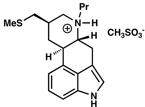
pergolide mesylate
