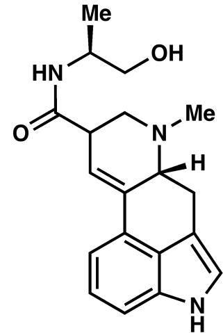
methysergide
