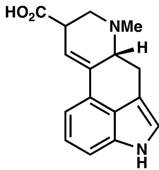
lysergic acid
